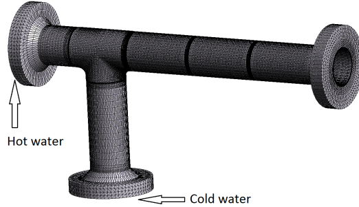
Figure 3.5: Mesh of the shut down nuclear reactor cooling loop.
