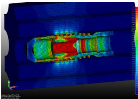
Figure 1.5: Constraint field after the plug insertion.
