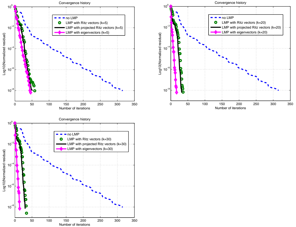
Figure 2.8: Mechanical bearing (linear case): convergence history of GMRES(30). Four preconditioning methods are compared: no second level preconditioning, limited memory preconditioners based on k = 5, 20 or 30 Ritz vectors, projected Ritz vectors and exact eigenvectors, respectively.
