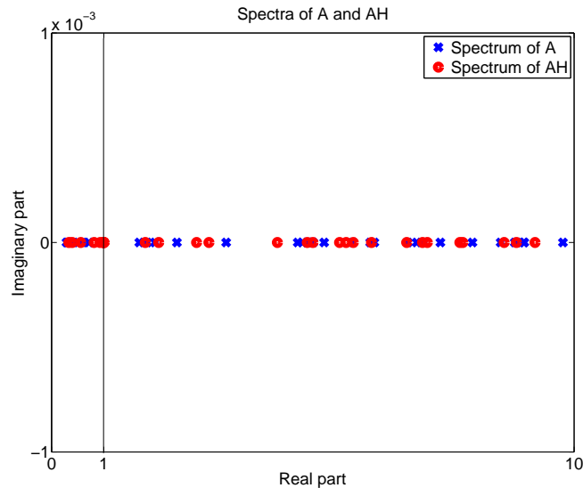
Figure 2.1: Eigendistribution of A and AH : case of 1 \in [\sigma_1, \sigma_N] .
