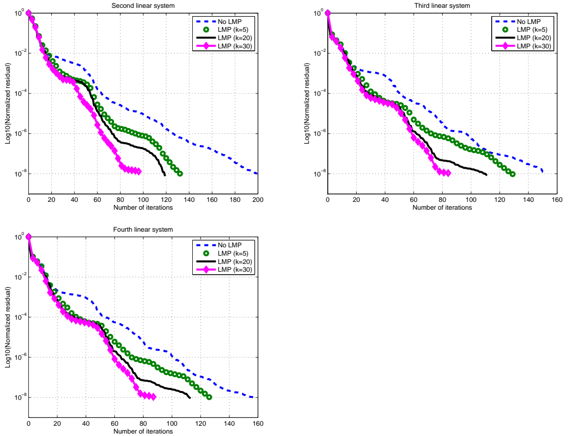
Figure 2.10: Containment building: convergence history of preconditioned GMRES(30) for the last three linear systems in the sequence. Case of limited memory preconditioners with k = 5, 20 or 30 Ritz vectors.
