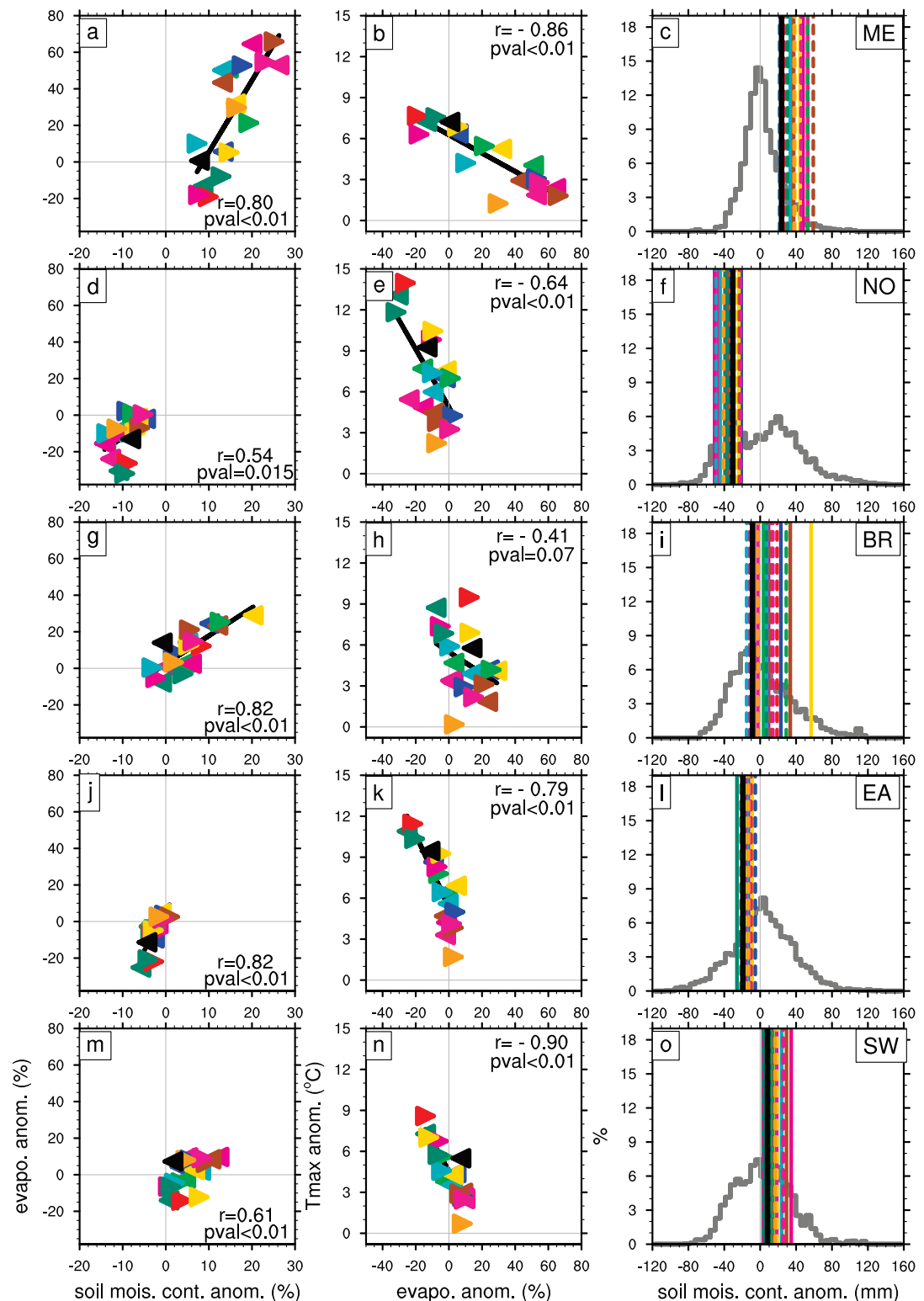
Figure 5. Scatter plots of the (relative, %; except for T_{max} , ^{\circ}C ) mean anomalies in (a,d,g,j,m) evapotranspiration and soil moisture, (b,e,h,k,n) T_{max} and evapotranspiration, in the reduced 19-member ALADIN-LE ensemble (black corresponds to ALADIN-SCEN). The regression line, value of the Spearman's rank correlation ( r ) and associated p -value are indicated on each panel. Mean anomalies in soil moisture (mm) in the reduced 19-member ALADIN-LE ensemble (vertical lines), compared to the probability density function of the climatological anomalies. All the anomalies are computed with regard to the 2061–2090 climatology. T_{max} and evapotranspiration anomalies are averaged during the first ten days of the heatwave (days 192–201), whereas soil moisture anomalies are averaged just before the heatwave to consider pre-existing conditions (days 184–188). All the anomalies are averaged across all the closest model grid points to each station (see figure S3) for each region in France (one per line as indicated; see figure 1).
