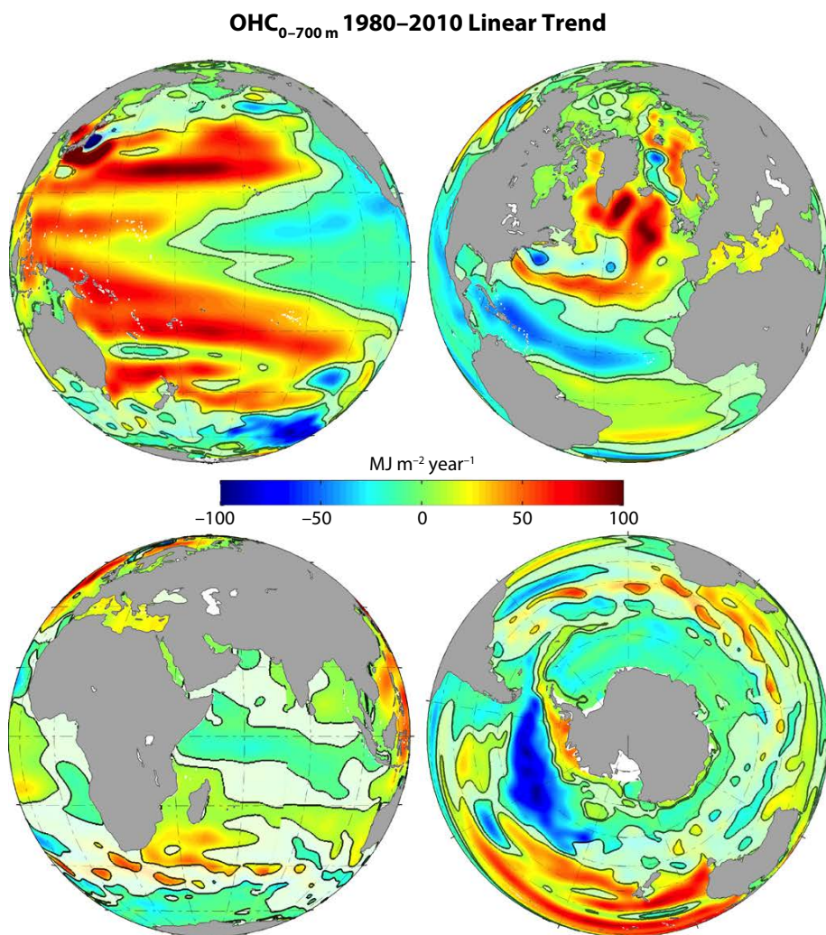
FIGURE 5. Forced linear trend of \text{OHC}_{0-700\text{m}} over 1980–2010 at scales larger than 1,000 km (colors) from four viewpoints. This forced trend is masked where it is smaller than twice the ensemble standard deviation. The spurious model trend was estimated from a climatological simulation and removed beforehand. Adapted from Sérazin et al. (2017)
