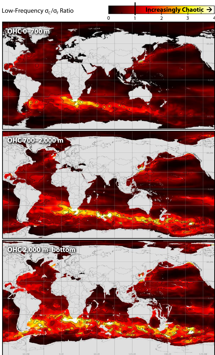
FIGURE 4. Ratio R between the chaotic and the forced interannual-to-decadal variabilities ( R = \sigma_C / \sigma_F ) of the large-scale OHC (scales larger than 1,000 km): from top to bottom, layers 0–700 m, 700–2,000 m, and 2,000 m–bottom. All time scales longer than about 15 years (hence, the trends) were first removed from the 50-member yearly OHC fields in the three layers using the nonparametric LOcal regrESSion (LOESS) method. Adapted from Sérazin et al. (2017)
