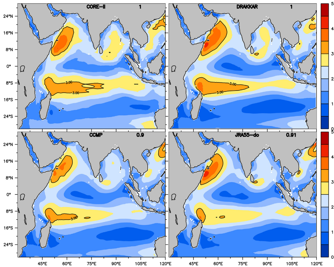
Fig. 3b. Monthly standard deviation (1993–2007) of wind speed (m/s) at 10 m height from CORE-II, DRAKKAR, CCMP and JRA55-do. The basin averaged mean values are given in the upper right corner of each panel.
