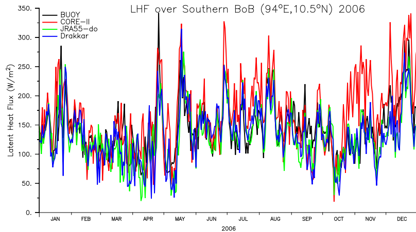
Fig. 4. Latent Heat Flux (LHF) computed from buoy observations (black) and replaced buoy wind speed with CORE-II (red curve), JRA55-do (green curve) and DRAKKAR (blue curve) wind speed fields. In the calculation of LHF only wind fields are changed, while all other fields are from observations. This comparison reveals the impact of wind speed on LHF.
