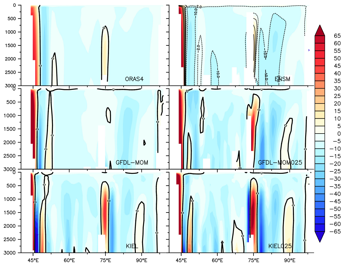
Fig. 32b. Transport across the equator from MOM, MOM025, KIEL, KIEL025, all model ensemble and ORAS4 in July. Units are in \text{m}^2/\text{s} .
