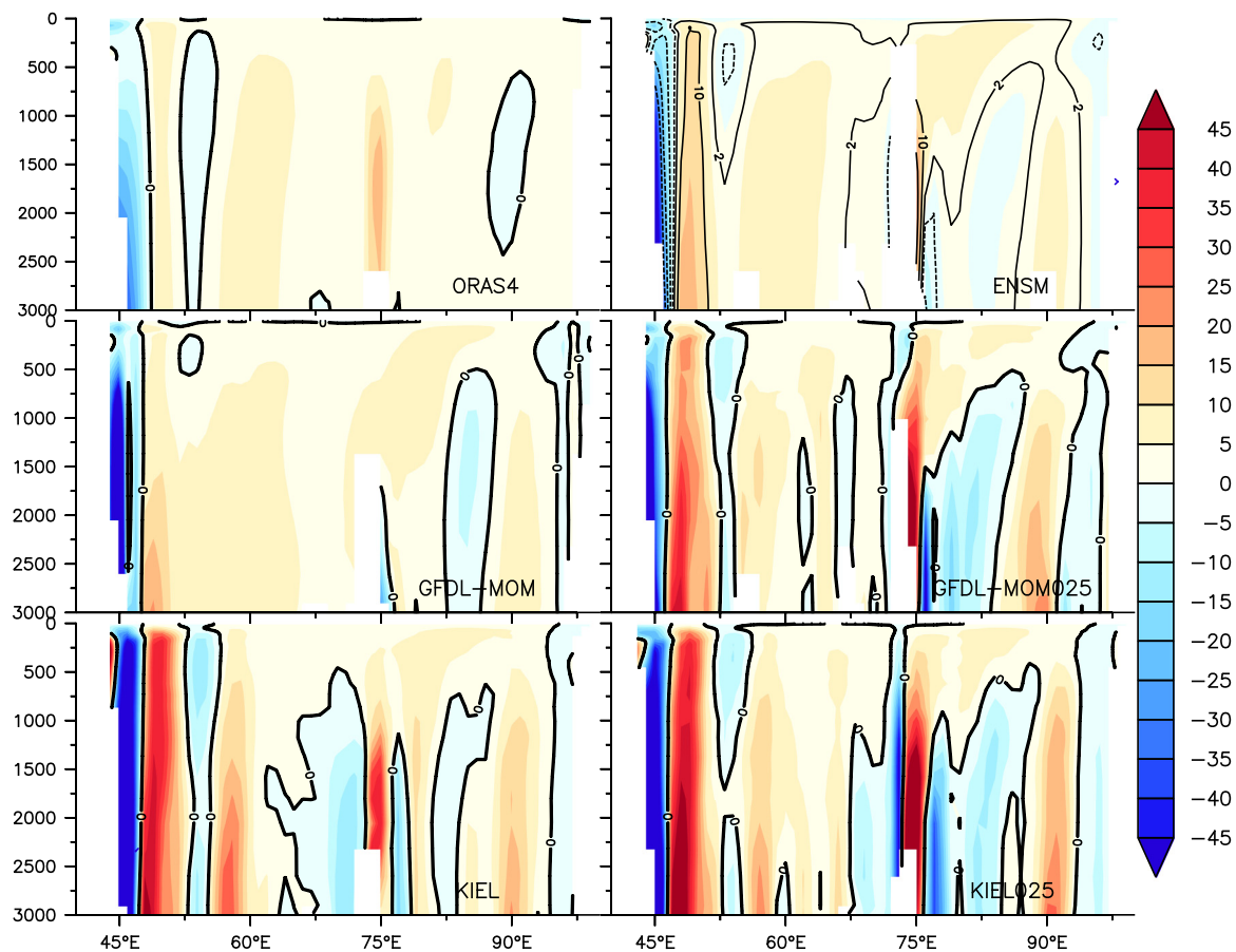
Fig. 32a. Transport across the equator from MOM, MOM025, KIEL, KIEL025, all model ensemble and ORAS4 in January. Units are in \text{m}^2/\text{s} .
