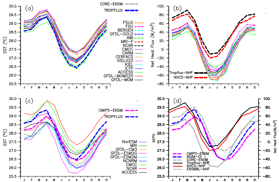
Fig. 13. Same as Fig. 10 but for the Thermocline Ridge (TR) region.
