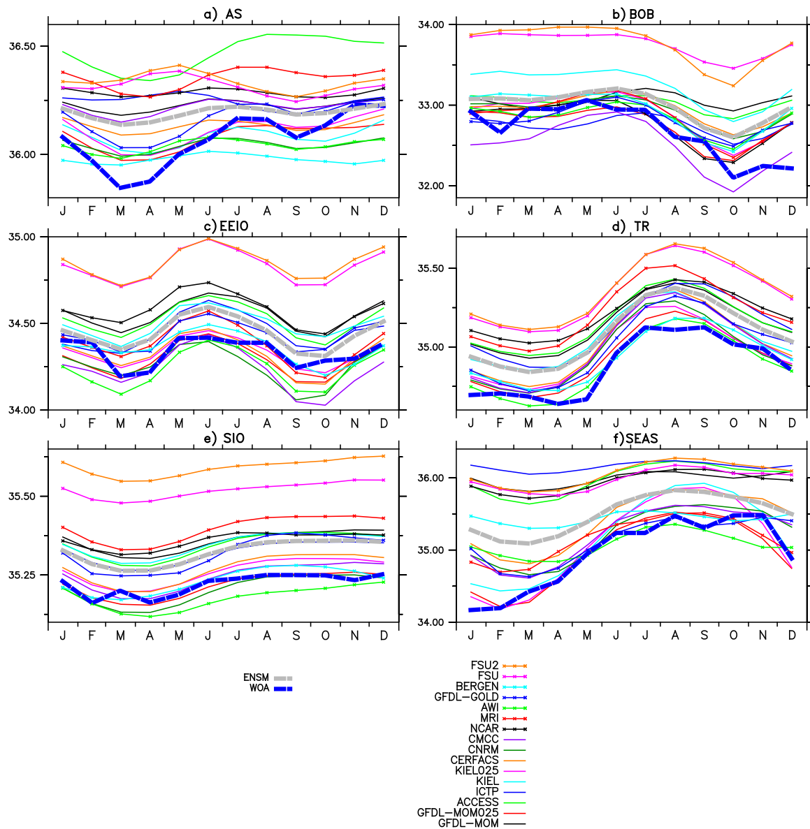
Fig. 16. Seasonal cycle of sea surface salinity from all CORE-II models and WOA observation over different sub-regions of the Indian Ocean (see Section 3.4 for sub-regional specifications).
