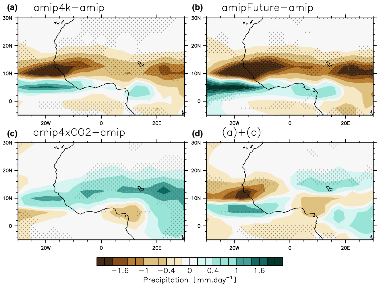
Fig. 8 Difference in July–September ensemble mean precipitation ( \text{mm}\cdot\text{day}^{-1} ) between a the CMIP5 amip4K and amip, b amipFuture and amip, c amip4xCO2 and amip simulations. d Sum of the
